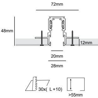
M19A Trimless Recessed Track
