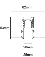
1.5M/2M M19T Embedded
