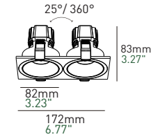
Double GA75-R01QS (with plate M-GA01-K02)
